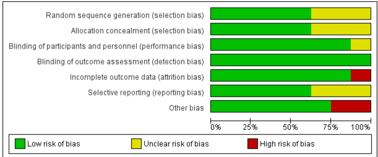
6 Figure 2: Risk of bias graph: review authors' judgement about each risk of bias item 7 presented as percentages across all included studies
