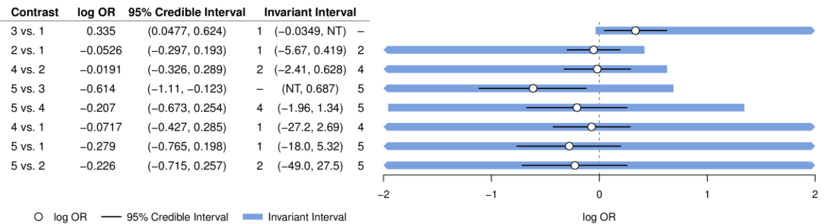
7 Figure 70: Contrast level threshold analysis for the mortality prior to discharge 8 outcome, for the worst ranked treatment. The smallest threshold 9 corresponds to a reduction in the log odds ratio of 3 vs. 1 of -0.37.
