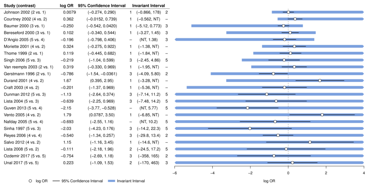
2 Figure 67: Study level threshold analysis for the BPD outcome, for the worst ranked 3 treatment. Moderately large changes in the odds ratios of BPD would be 4 required for the worst ranked treatment to change, with the smallest being a 5 reduction in the log odds ratio of the Johnson 2002 study of -0.87.
