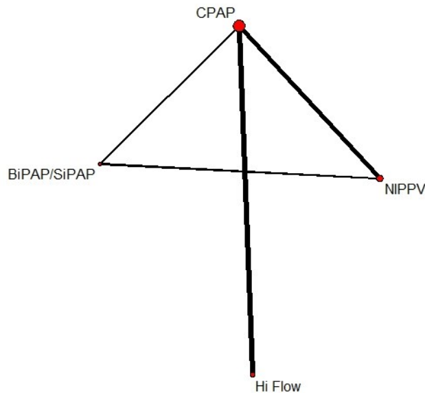
1 Figure 58: Network diagram of comparisons for which direct evidence on mortality 2 prior to discharge was available
