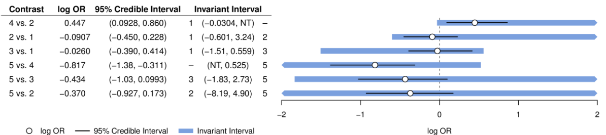
10 Figure 66: Contrast level threshold analysis for the BPD outcome, for the worst ranked 11 treatment. Moderately large changes in the odds ratios of BPD would be 12 required for the worst ranked treatment to change, with the smallest being a 13 reduction of -0.48 in the log odds ratio of the 4 vs. 2 contrast.
