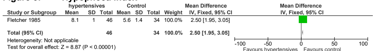
Figure 3: Hypopnoea index
