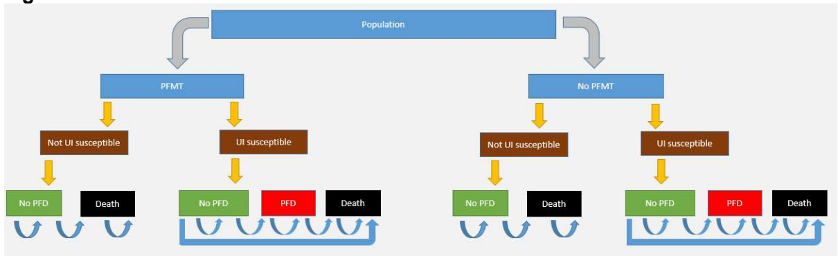
Figure 4: Schematic of Markov decision model
