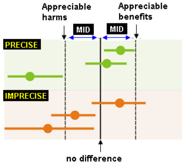
1 Figure 3.1: Illustration of precise and imprecise outcomes based on the confidence interval of 2 outcomes
