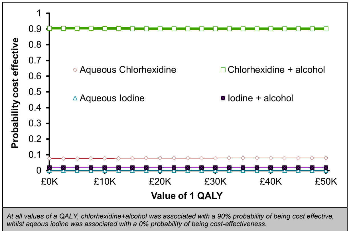
1 2 Figure HE19. Cost-effectiveness acceptability curve for where Chlorhexidine + Alcohol costs = Hydrex
