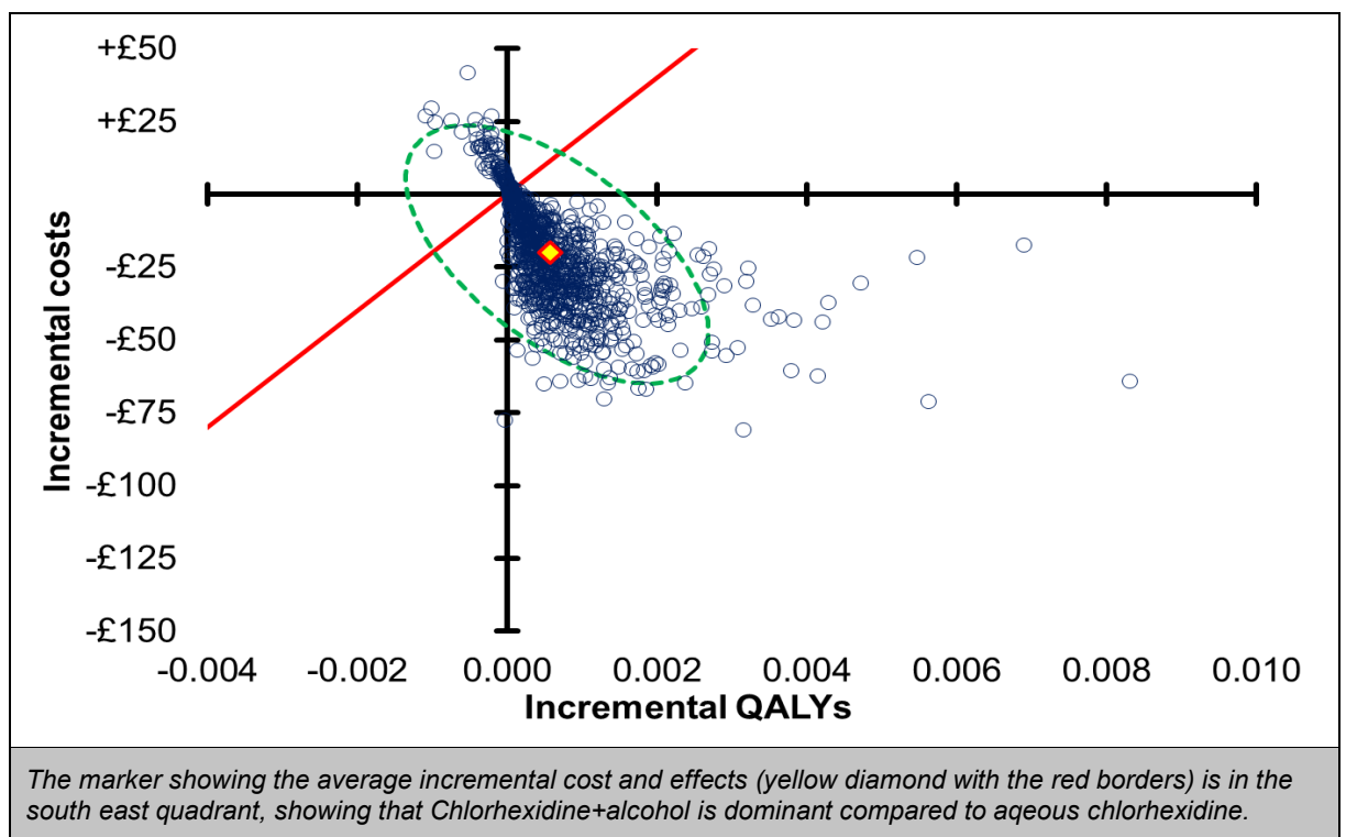
3 4 5 Figure HE22. Probabilistic sensitivity analysis comparison of Chlorhexidine + Alcohol vs Chlorhexidine + Aqueous for where Chlorhexidine + Alcohol costs = ChloroPrep, 5,000 iterations
