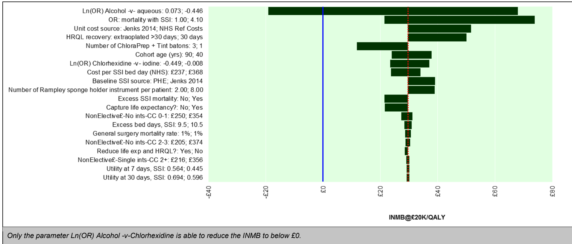
1 Figure HE14. One-way sensitivity analysis for chlorhexidine + alcohol vs aqueous chlorhexidine where chlorhexidine + alcohol costs = 2 ChloraPrep+Tint - INBM @ £20k per QALY
