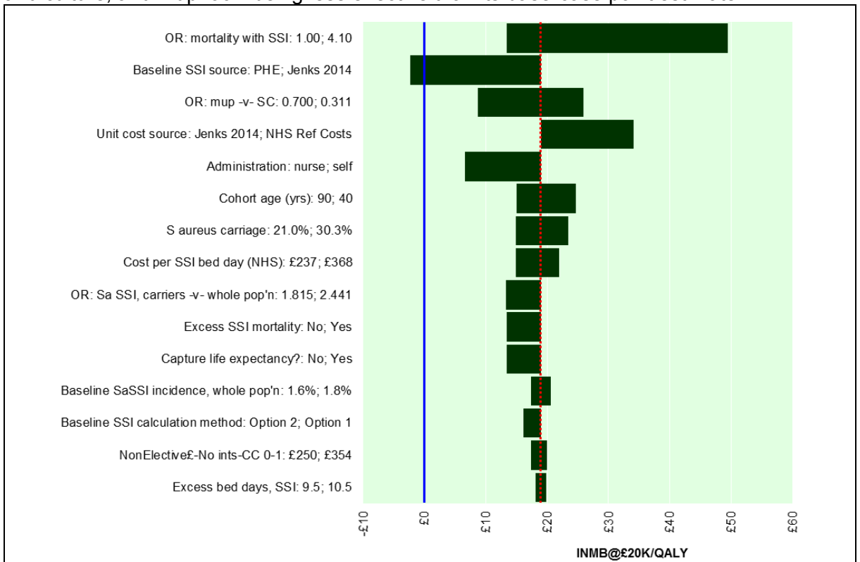
16 Figure HE04: One-way sensitivity analysis results (all surgery cohort) – universal 17 mupirocin vs. standard care (no nasal decolonisation)
