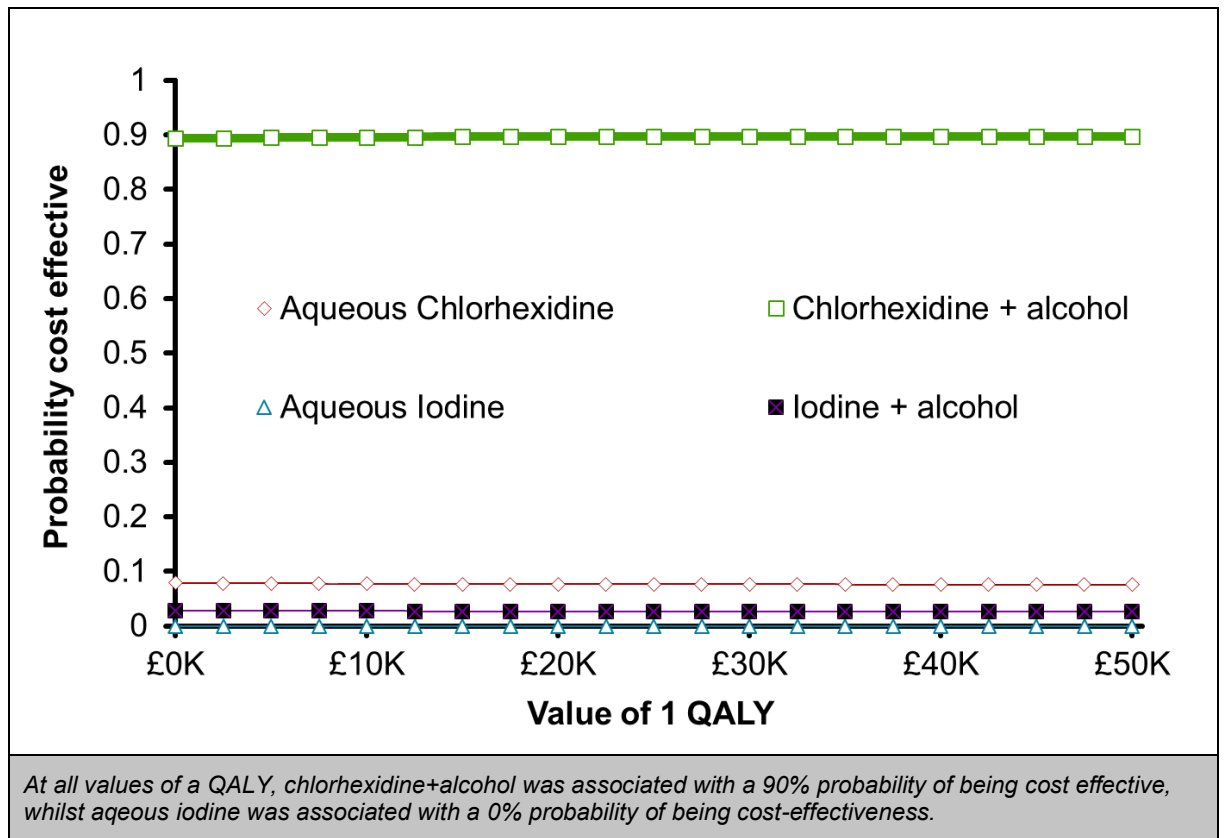
1 Figure HE17. Cost-effectiveness acceptability curve for where Chlorhexidine + Alcohol 2 costs = 2% Ecolab
