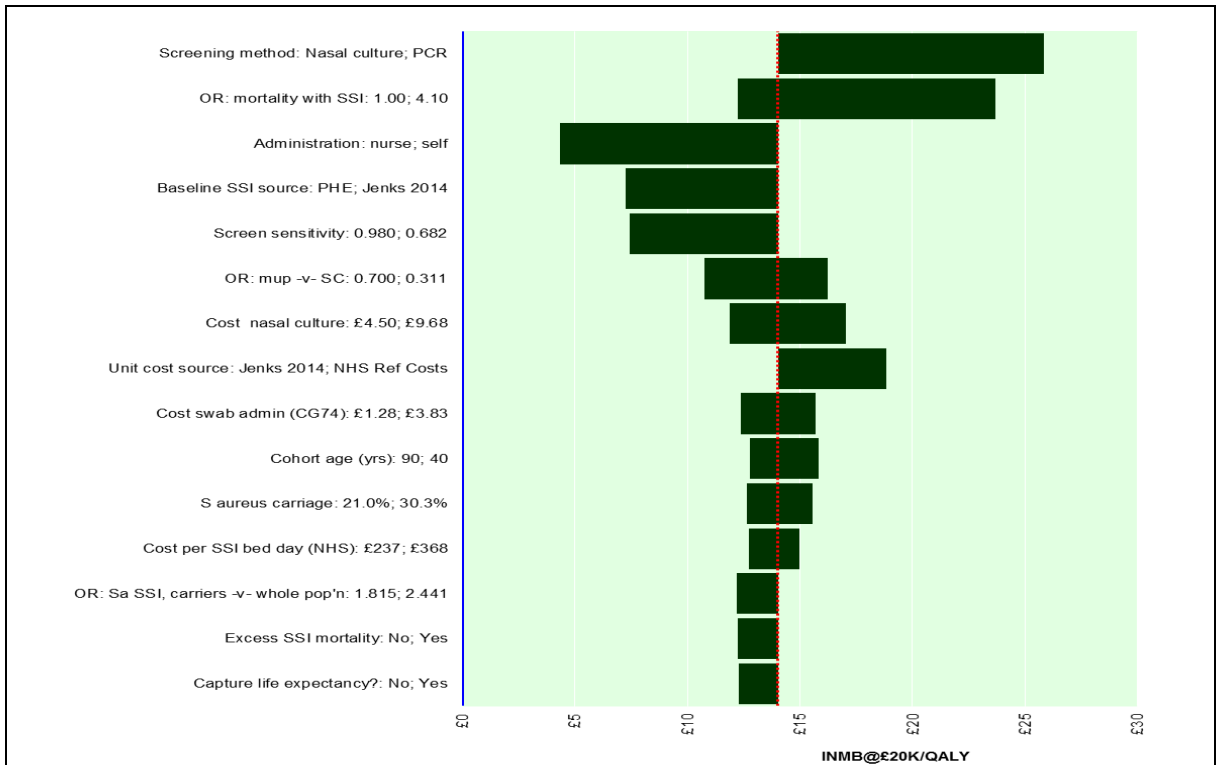
1 Figure HE05: One-way sensitivity analysis results (all surgery cohort) – universal 2 mupirocin vs. screen & treat if positive
