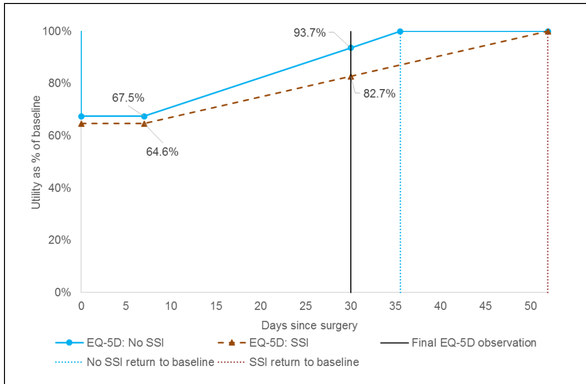
3 Figure HE02: Short-term quality of life recovery with and without SSI
