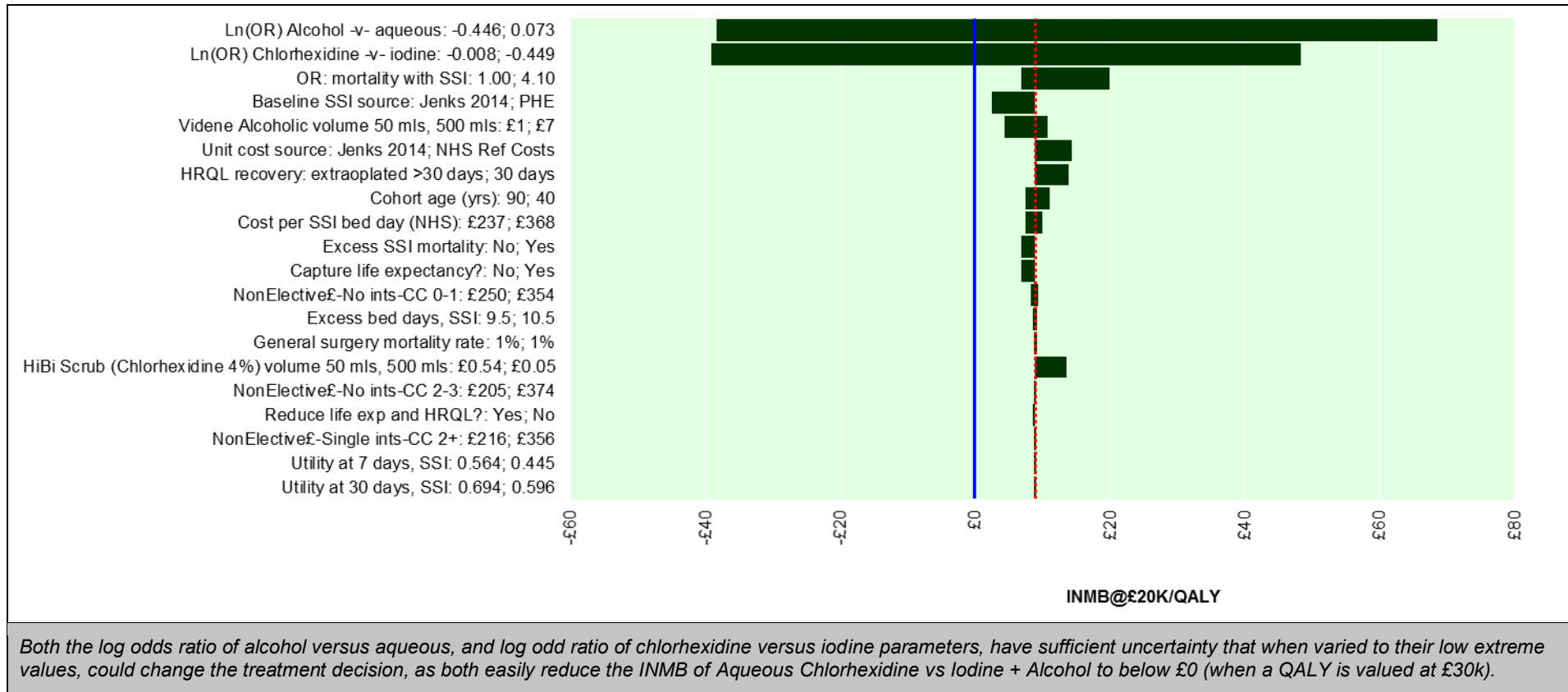
1 Figure HE16. One-way sensitivity analysis for aqueous chlorhexidine vs iodine + alcohol - INBM @ £20k per QALY
