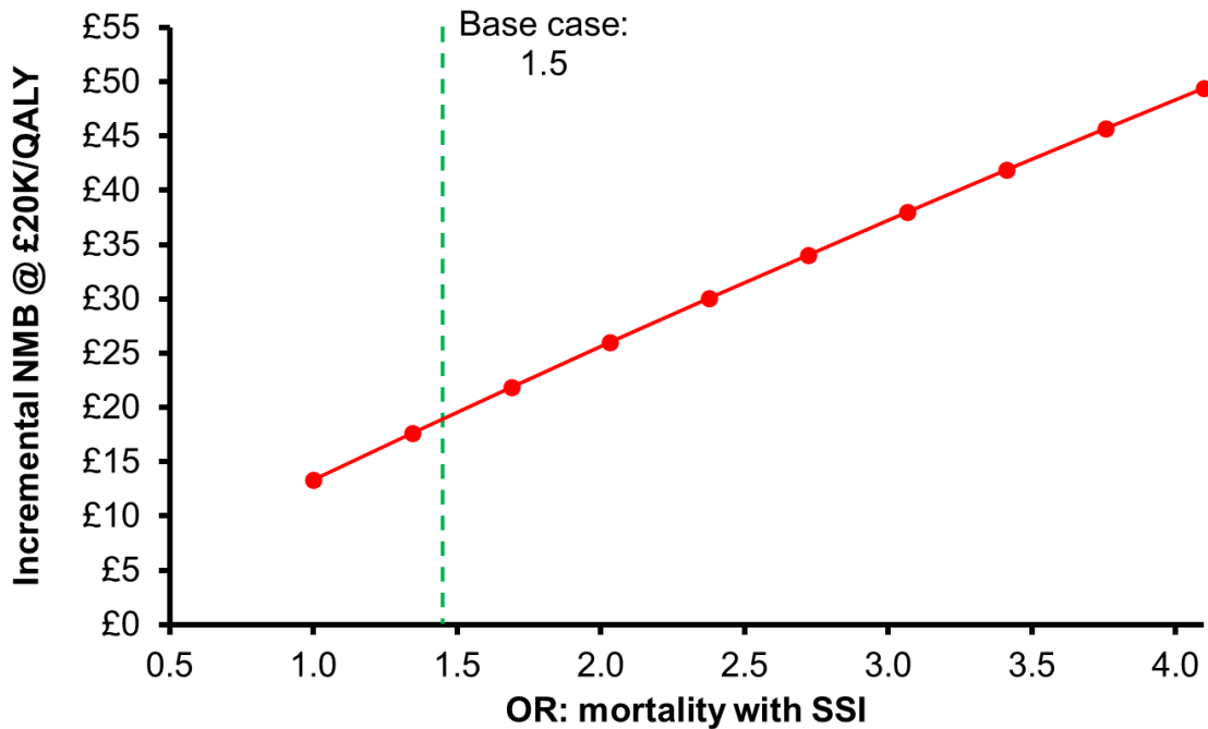
9 Figure HE09. Pairwise threshold analysis of the universal mupirocin vs standard care 10 at an INMB @ £20k/QALY where the odds ratio of mortality with an SSI is 11 varied
