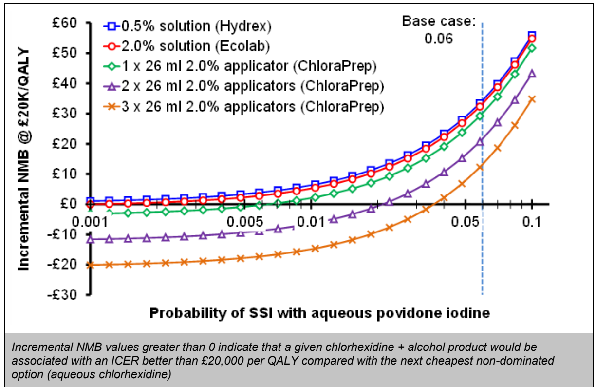
Figure HE25: One-way sensitivity analysis: cost effectiveness of chlorhexidine + alcohol as a function of baseline probability of SSI
