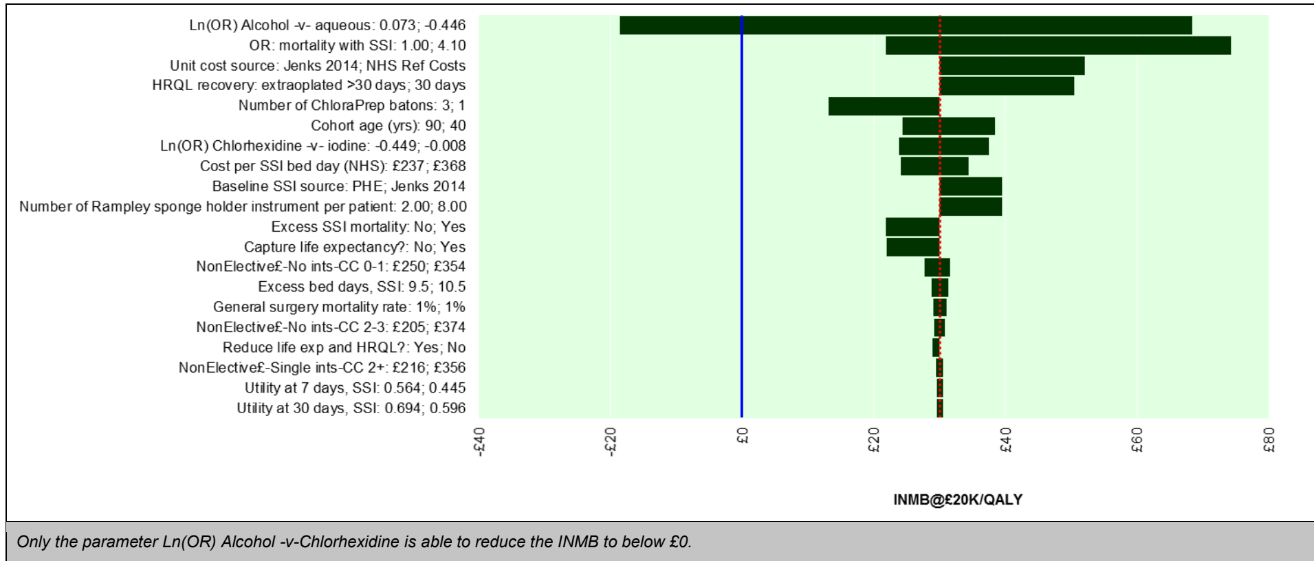
1 Figure HE13. One-way sensitivity analysis for chlorhexidine + alcohol vs aqueous chlorhexidine where chlorhexidine + alcohol costs = 2 ChloraPrep - INBM @ £20k per QALY
