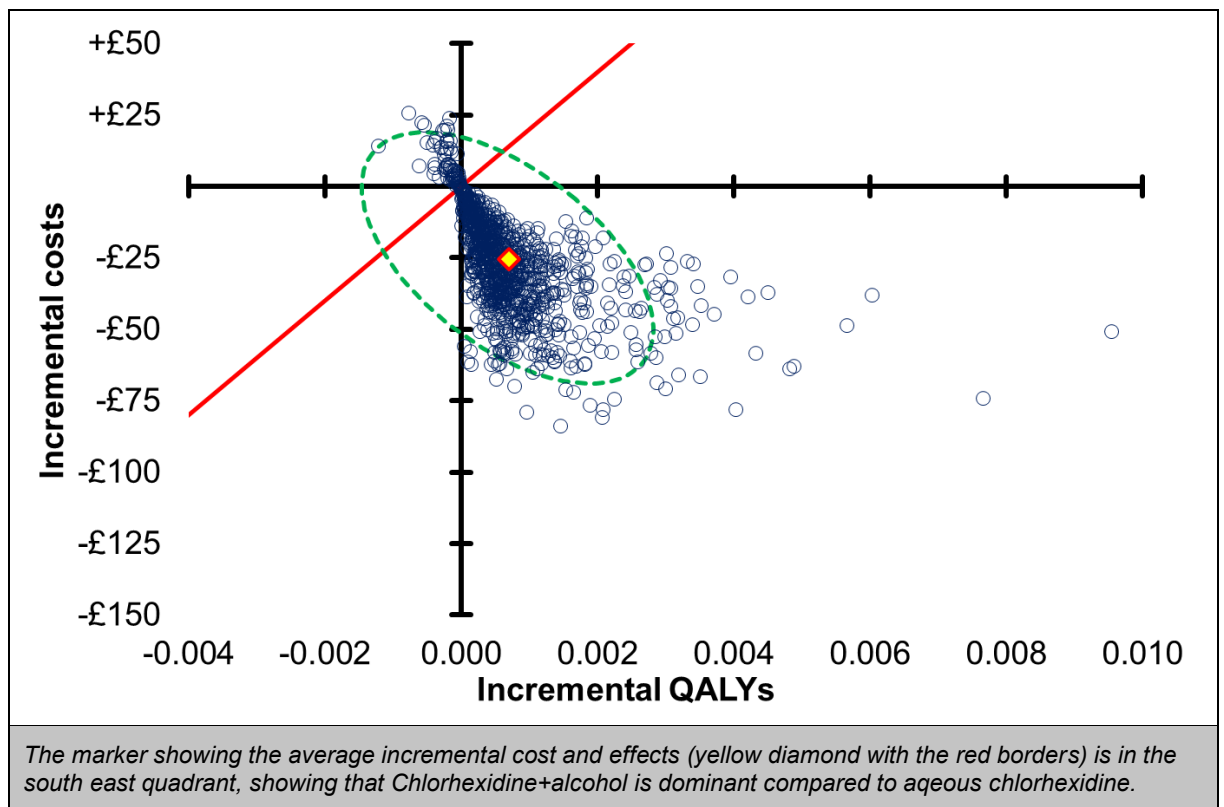
3 4 5 Figure HE20. Probabilistic sensitivity analysis comparison of Chlorhexidine + Alcohol vs Chlorhexidine + Aqueous for where Chlorhexidine + Alcohol costs = Hydrex, 5,000 iterations
