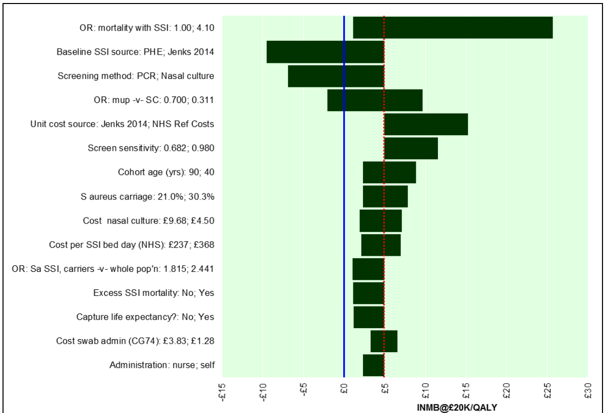
3 Figure HE06: One-way sensitivity analysis results (all surgery cohort) – screen & treat 4 if positive vs. standard care (no nasal decolonisation)
