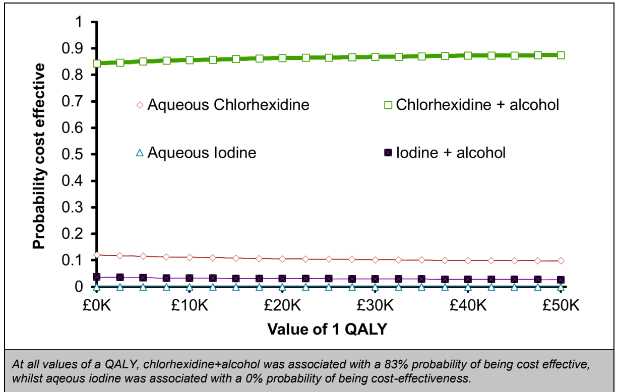
1 2 Figure HE21. Cost-effectiveness acceptability curve for where Chlorhexidine + Alcohol costs = ChloroPrep
