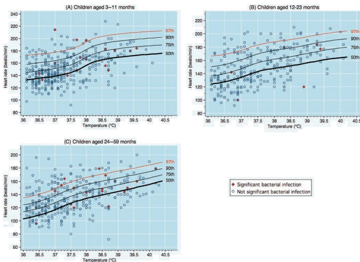
Figure 5.1 Temperature and pulse of children presenting to the emergency department with and without significant bacterial infection (Brent et al., 2011) (Reproduced under open access publishing agreements)
