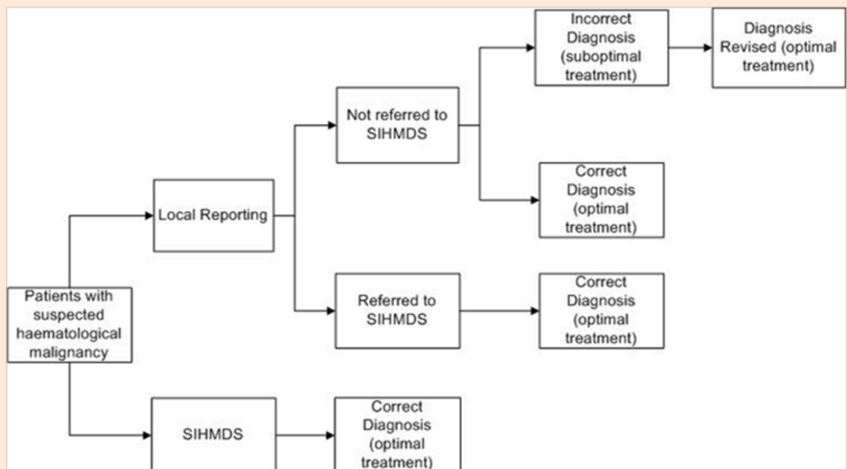
Figure 4: Model Structure
