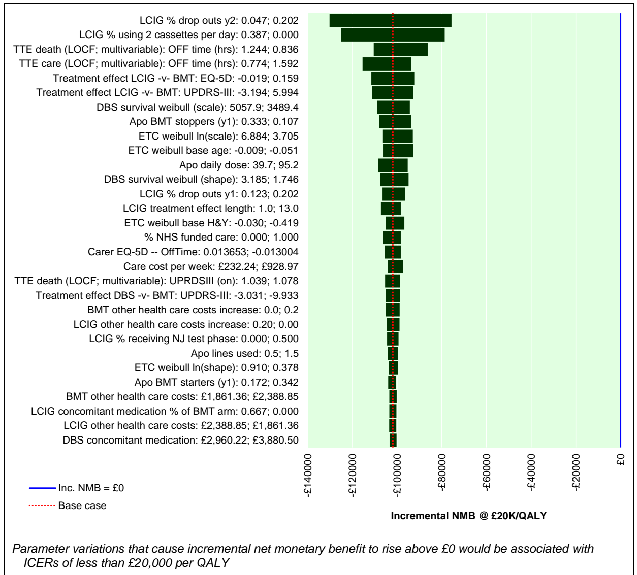
Figure 14: One-way sensitivity analysis – LCIG -v- BMT: 30 most influential parameters (using PINE LOCF models for time to full-time care and time to death; PINE extrapolation trajectories; PINE multiply imputed model for EQ-5D)
