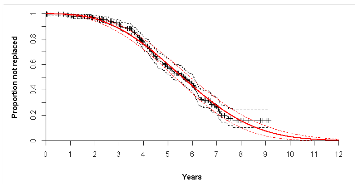
Figure 6: Original cost-utility model: time to replacement of IPG
