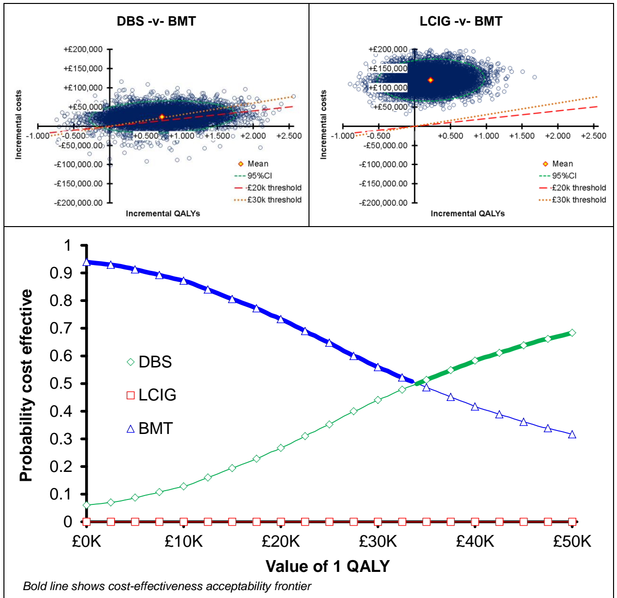
Figure 9: Original cost-utility model: probabilistic sensitivity analysis – incremental cost-utility scatterplots and cost-effectiveness acceptability curve and frontier
