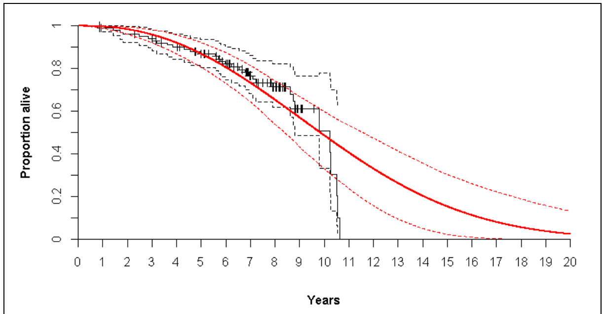
Figure 5: Original cost–utility model: baseline time-to-death function (PDSURG dataset [all HY≥3 participants undergoing DBS surgery, regardless of initial allocation]) with fitted Weibull function
