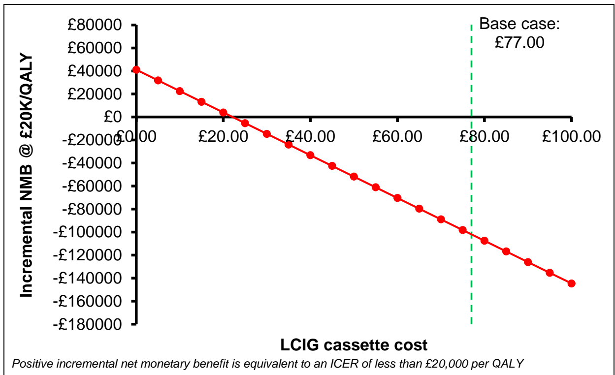
Figure 15: Detailed one-way sensitivity analysis for LCIG -v- BMT – cost per cassette of LCIG (using PINE LOCF models for time to full-time care and time to death; PINE extrapolation trajectories; PINE multiply imputed model for EQ-5D)
