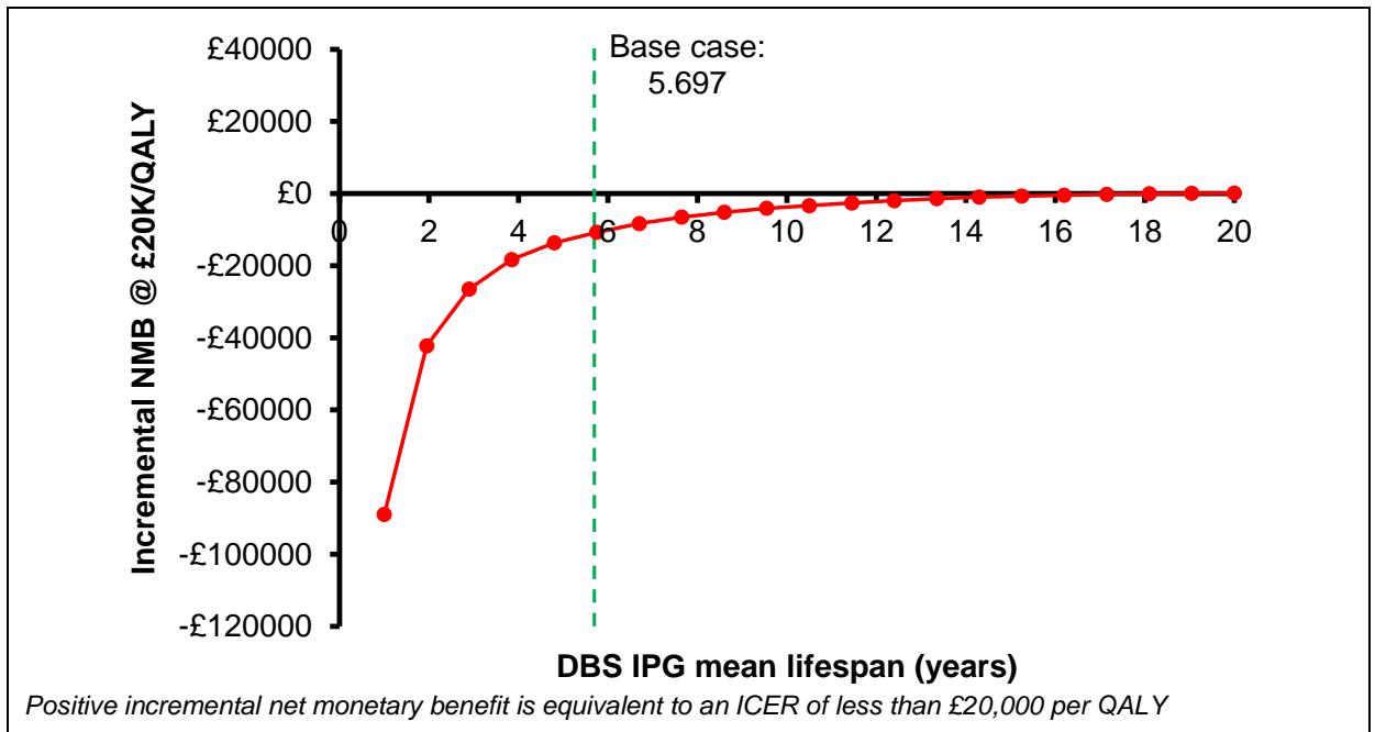
Figure 11: Detailed one-way sensitivity analysis for DBS -v- BMT – mean IPG battery lifespan (using PINE LOCF models for time to full-time care and time to death; PINE extrapolation trajectories; PINE multiply imputed model for EQ-5D)
