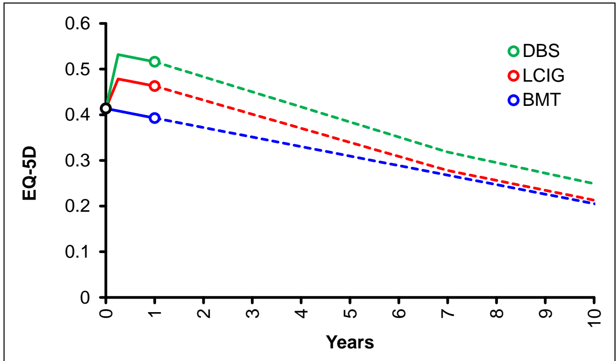
Figure 7: Extrapolated EQ-5D benefit over time when modelled as a function of other clinical variables rather than independently (cf. Figure 3)
