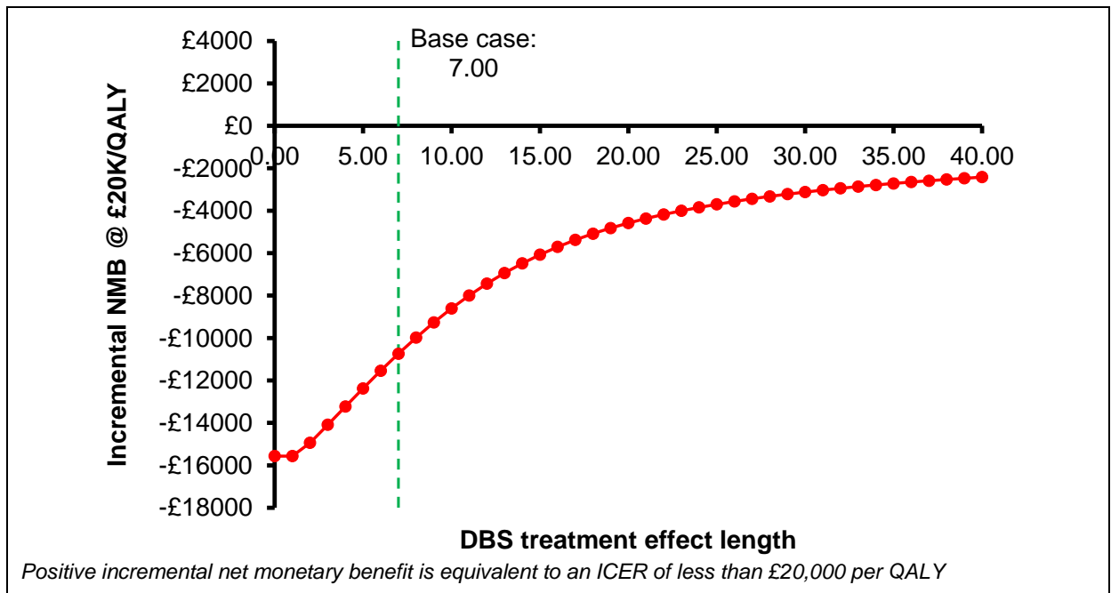
Figure 13: Detailed one-way sensitivity analysis for DBS -v- BMT – duration of treatment benefit (using PINE LOCF models for time to full-time care and time to death; PINE extrapolation trajectories; PINE multiply imputed model for EQ-5D)
