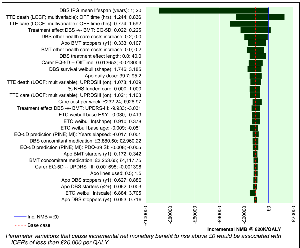
Figure 10: One-way sensitivity analysis – DBS -v- BMT: 30 most influential parameters (using PINE LOCF models for time to full-time care and time to death; PINE extrapolation trajectories; PINE multiply imputed model for EQ-5D)
