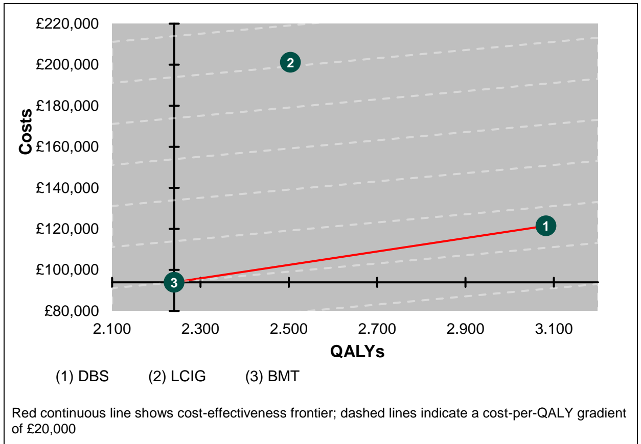
Figure 8: Original cost-utility model: cost-utility plane
