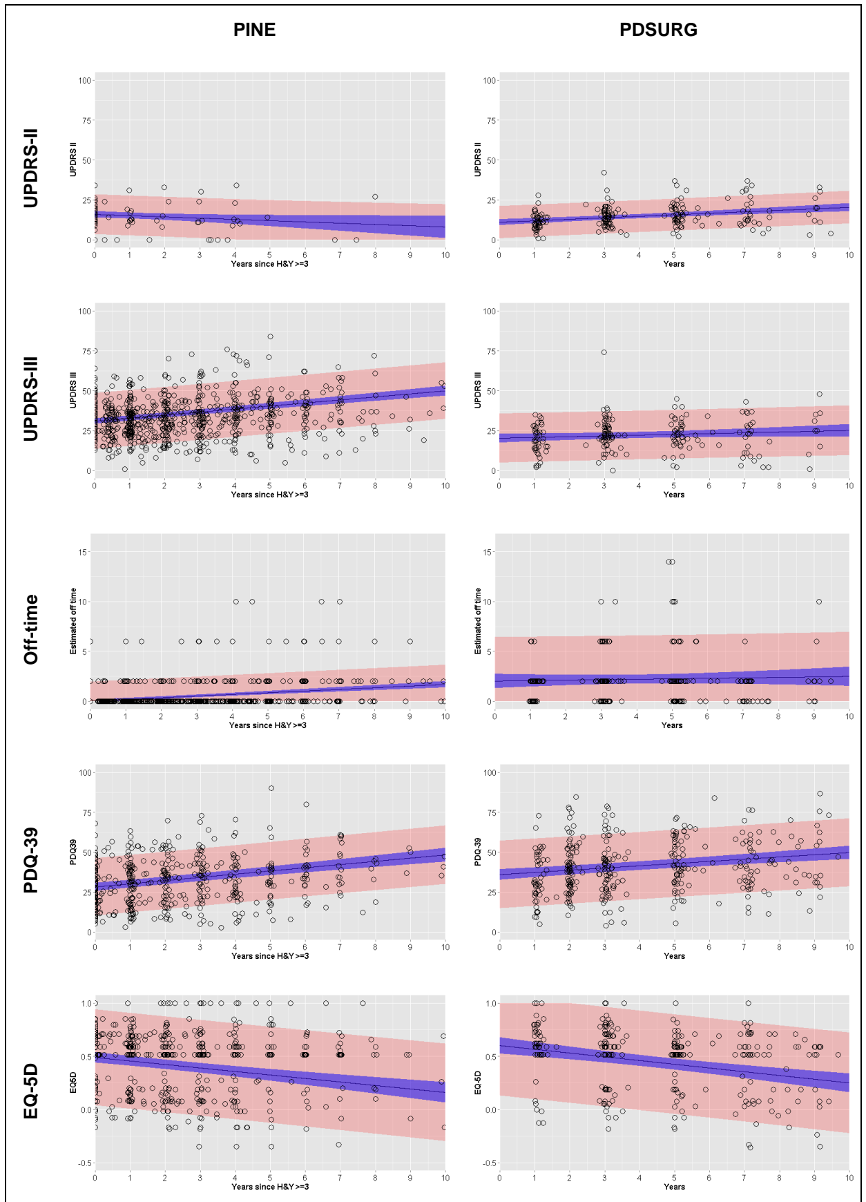
Figure 2: Original cost–utility model: trajectories for extrapolating clinical variables over time
