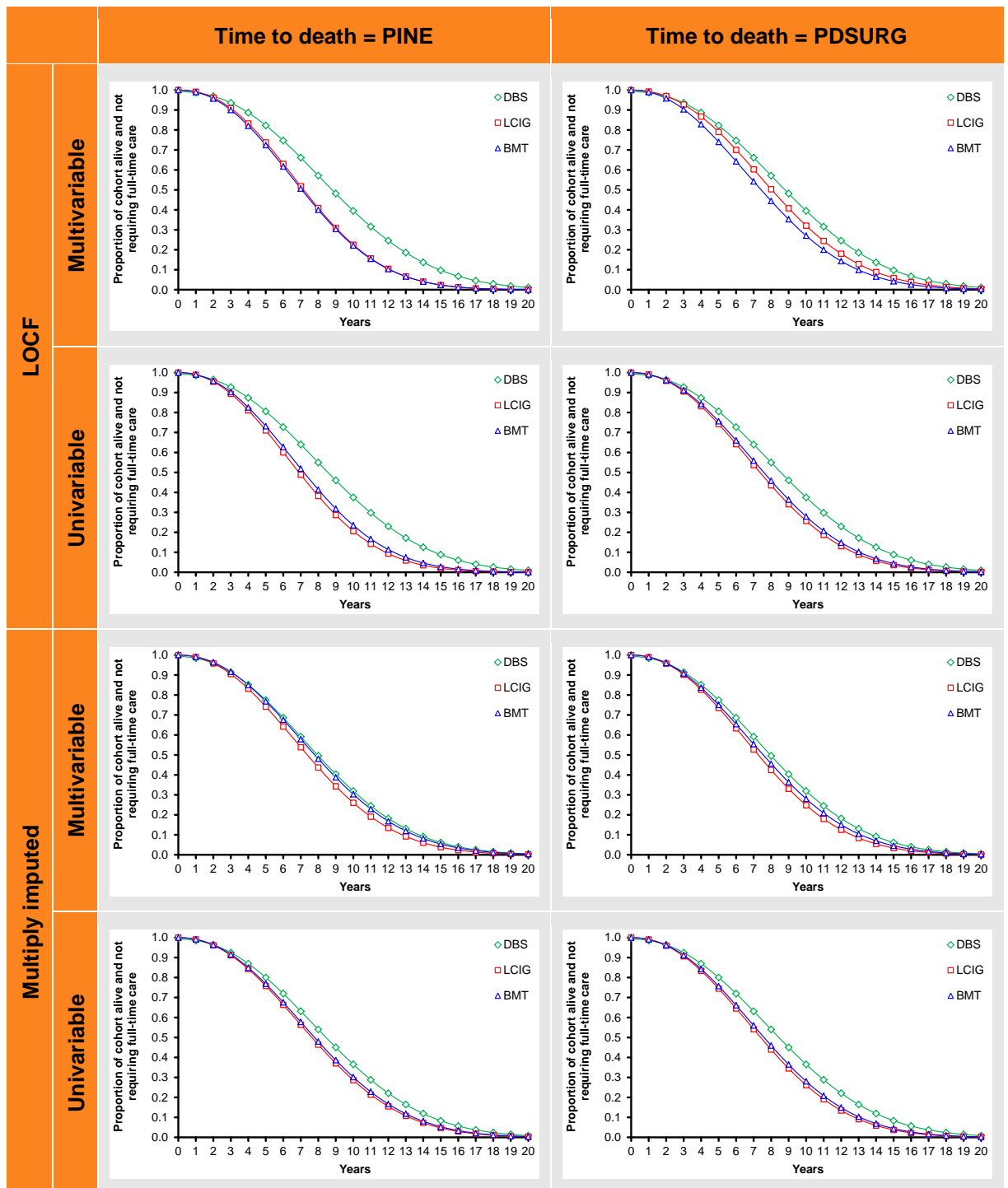
Figure 16: Original cost-utility model: predicted full-time-care-free survival according to choice of time-to-event models
