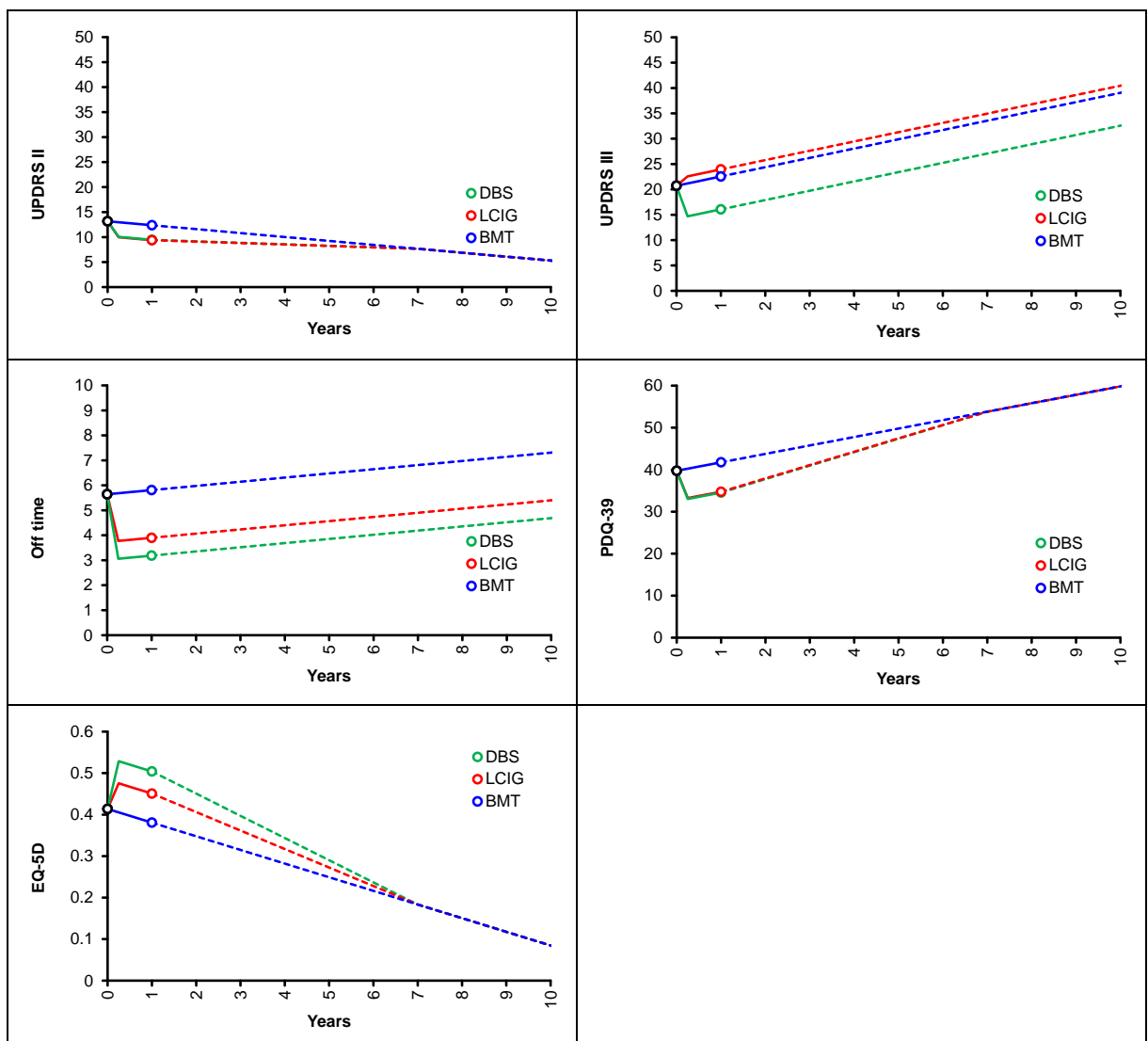
Figure 3: Diminishing (UPDRS-II; PDQ-39; EQ-5D) and constant (UPDRS-III; off-time) benefit over time in extrapolated treatment effects
