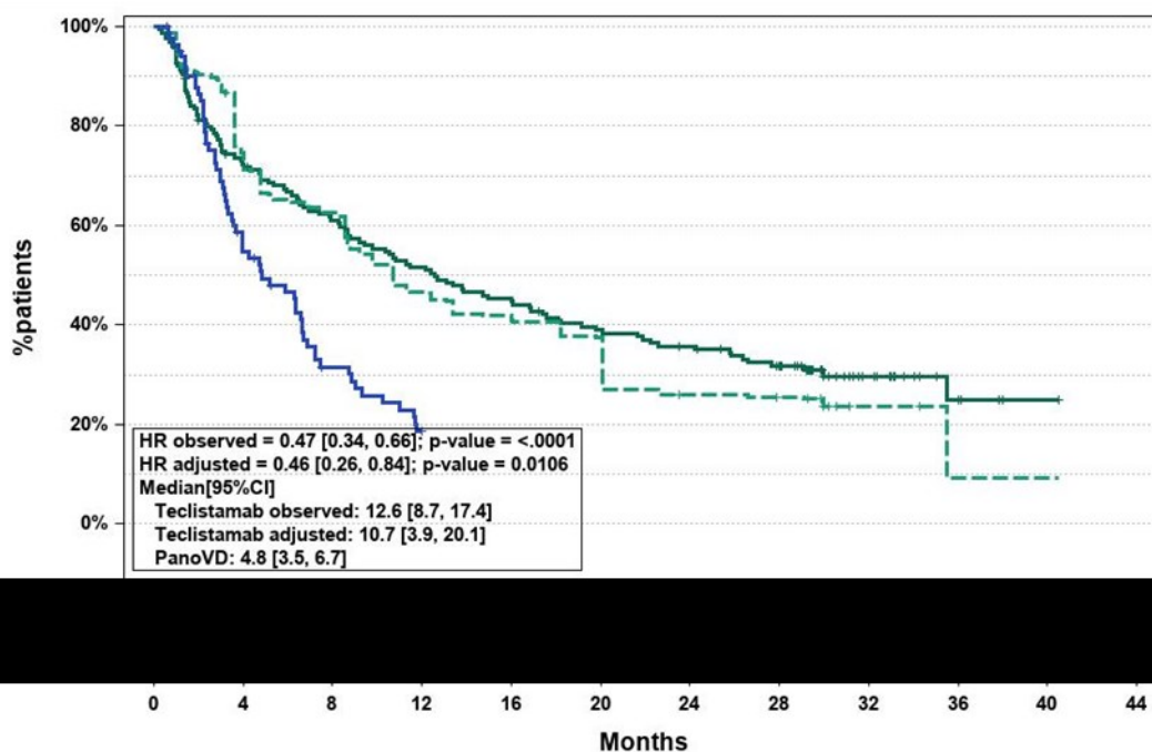
Figure 7: PFS KM curve (based on TTNT as a proxy) for teclistamab versus PanoBorDex (base case ITC)
