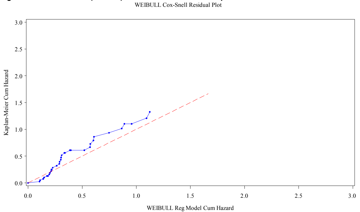
Figure 3-8 Brentuximab (no SCT) PFS – Cox-Snell residual plots – Weibull distribution
