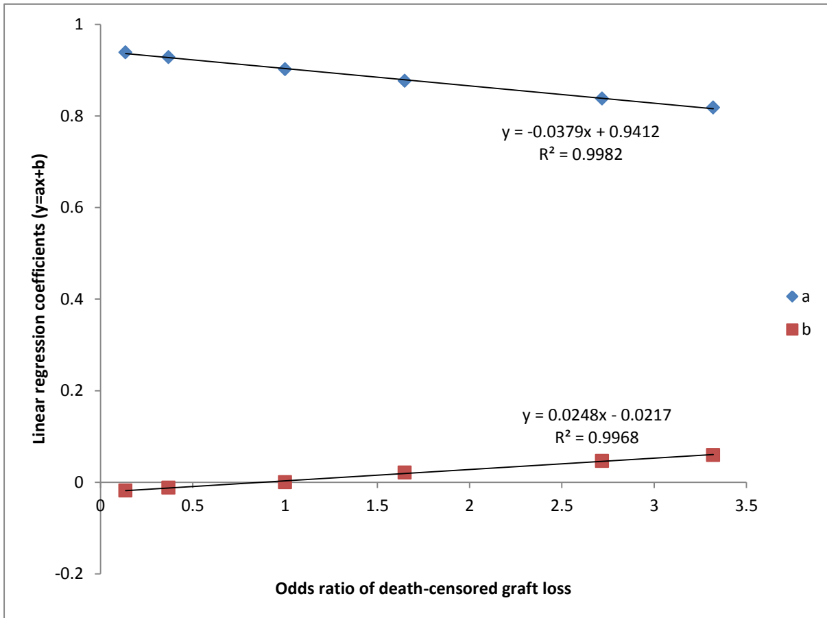
Figure 89. Linear regression coefficients for \ln(\text{odds ratio of patient death}) vs. \ln(\text{hazard ratio of death with functioning graft}) plotted versus odds ratio of graft loss
