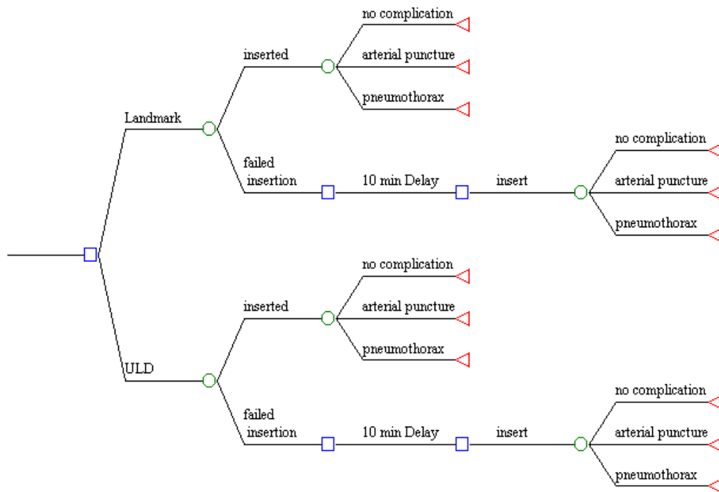
FIGURE 1. DECISION TREE
