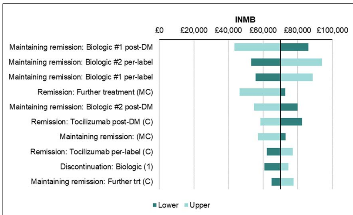
Figure 5 Tornado diagram – per-label arm versus no-anakinra arm
