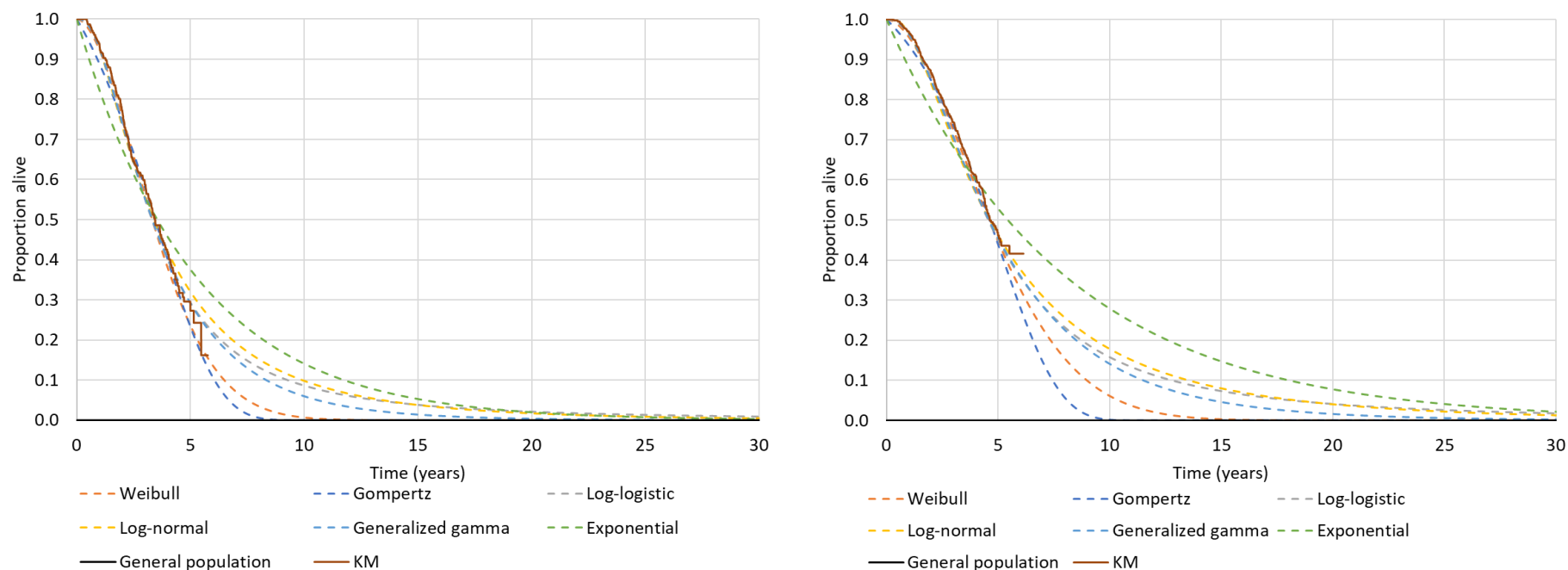
Figure 9: Fitted parametric models (Adjusted PFS2; SPARTAN) ADT alone (left) and apalutamide plus ADT (right)
