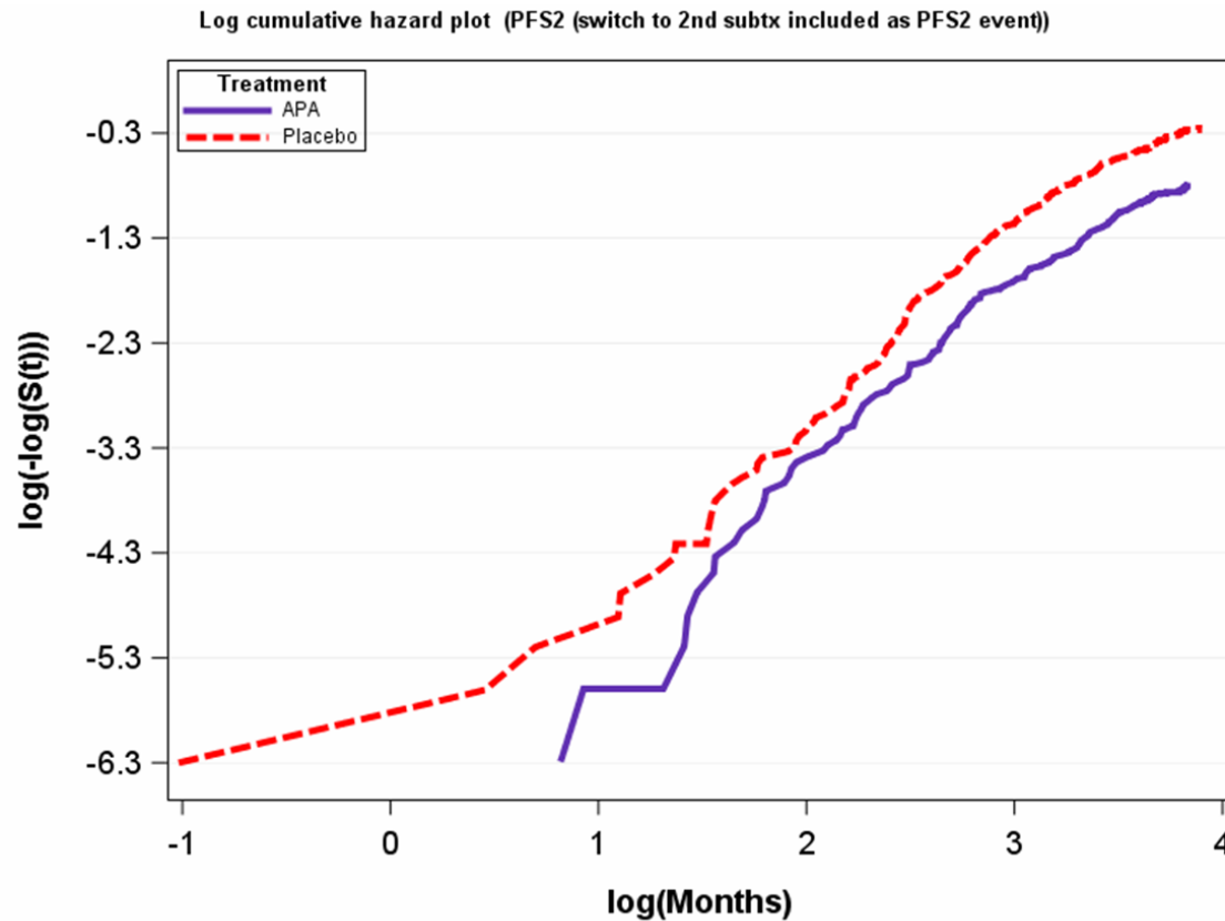
Figure 19: Log cumulative hazard plot for unadjusted PFS2 in TITAN (Final analysis, clinical cut-off date 7 September 2020, ITT population)
