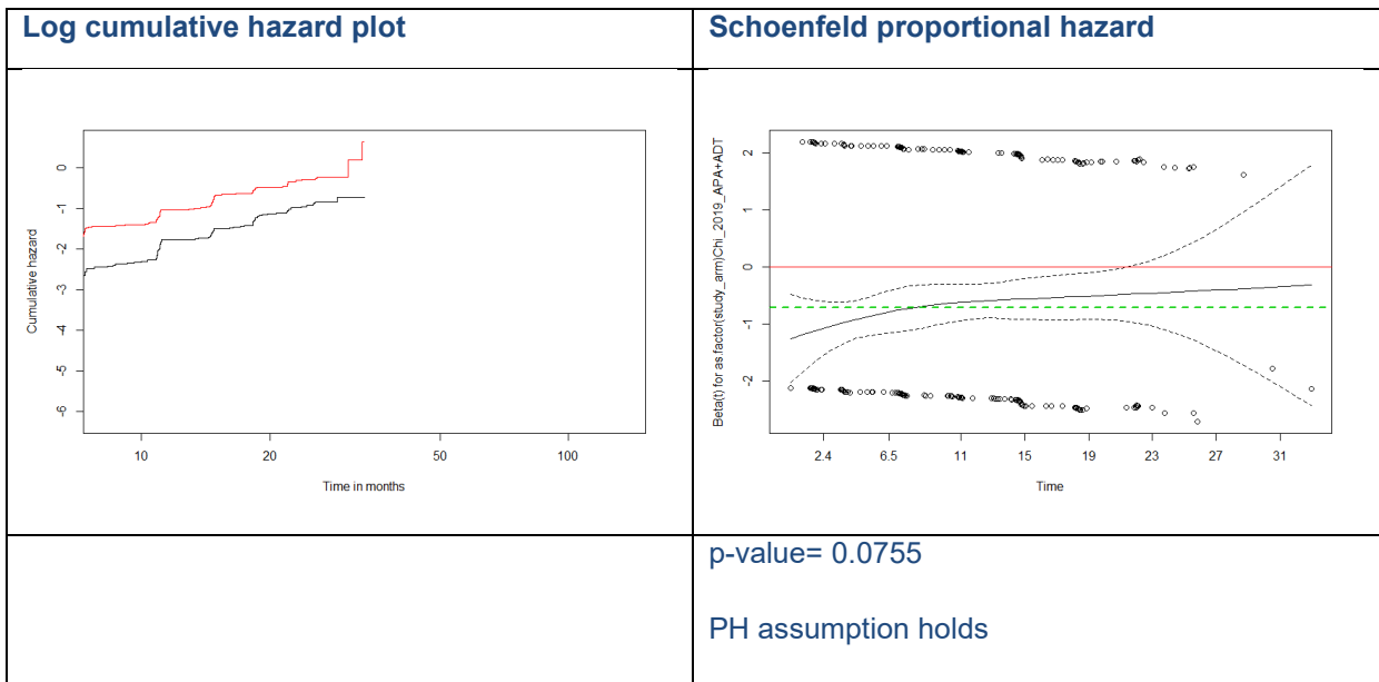
Figure 2: rPFS PH assessment for TITAN, apalutamide plus ADT versus placebo plus ADT (Chi 2019)
