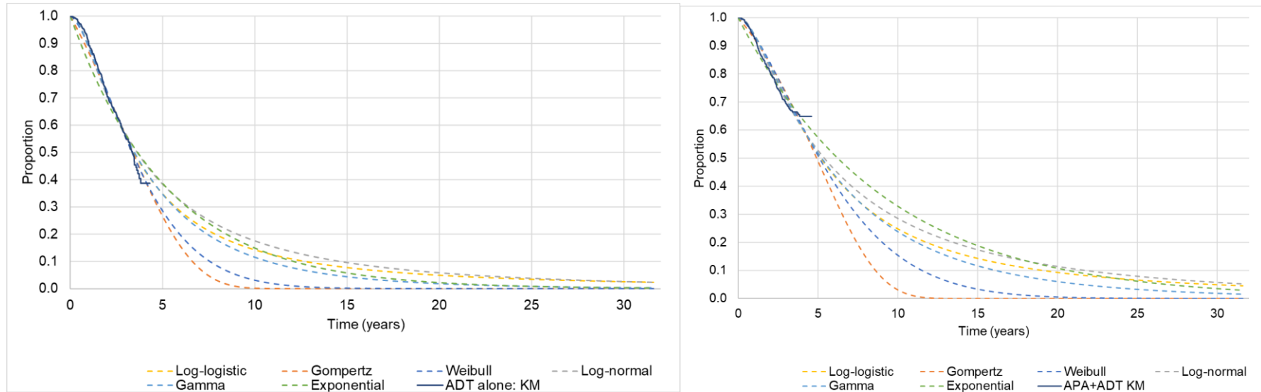
Figure 29. Jointly fitted parametric models (PFS2 adjusted using RPFSTM COU-AA-302 FA; TITAN final analysis) ADT alone (left) and apalutamide plus ADT (right)
