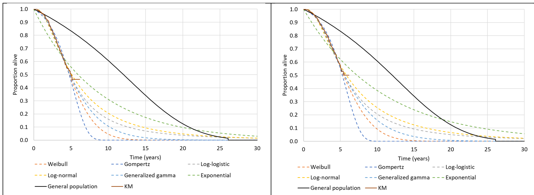
Figure 8: Fitted parametric models (adjusted OS, SPARTAN): ADT alone (left) and apalutamide plus ADT (right)
