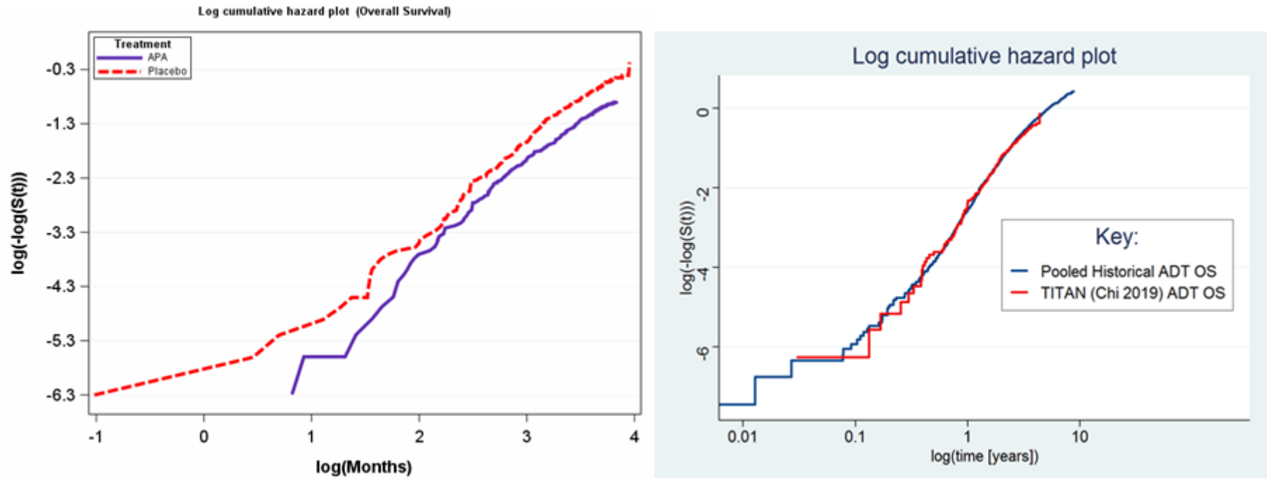
Figure 22: Log-cumulative hazard plots (overall survival: TITAN apalutamide plus ADT vs ADT alone, and TITAN ADT alone vs pooled historical ADT)
