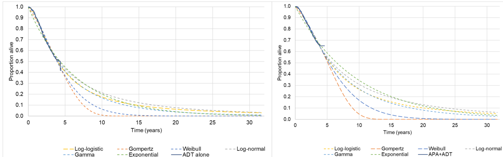
Figure 28. Jointly fitted parametric models (OS unadjusted; TITAN final analysis) ADT alone (left) and apalutamide plus ADT (right)
