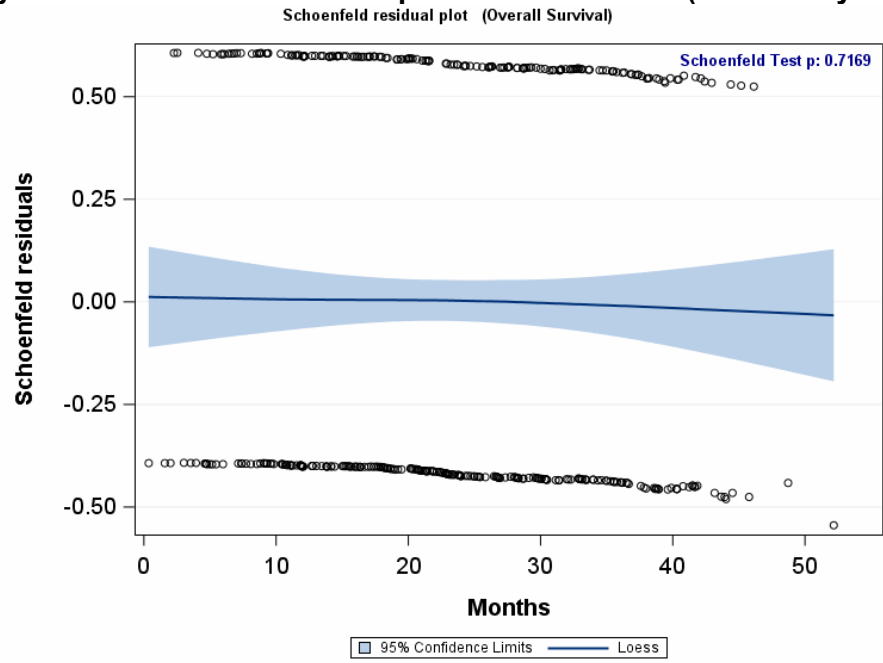
Figure 11. Schoenfeld residual plot for OS in TITAN (Final Analysis, clinical cut-off date 7 September 2020, ITT population)
