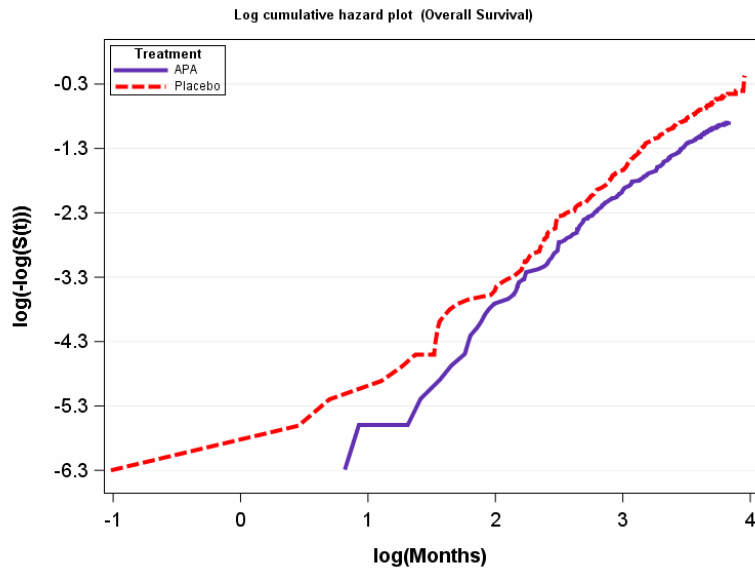
Figure 10. Log cumulative hazard plot for OS in TITAN (Final analysis, clinical cut-off date 7 September 2020, ITT population)
