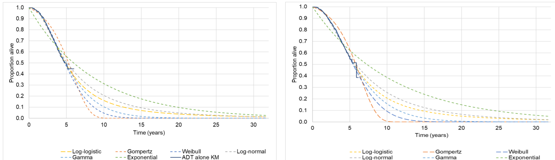
Figure 26. Jointly fitted parametric models (OS adjusted using RPFSTM COU-AA-302 IA3; SPARTAN final analysis) ADT alone (left) and apalutamide plus ADT (right)
