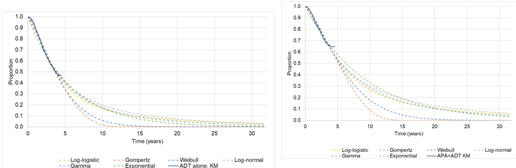
Figure 27. Jointly fitted parametric models (PFS2 unadjusted; TITAN final analysis) ADT alone (left) and apalutamide plus ADT (right)
