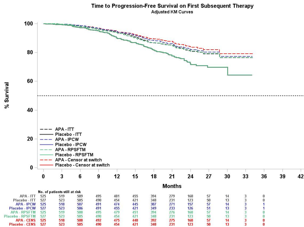
Figure 10: TITAN Observed and Adjusted PFS2 KM curves
