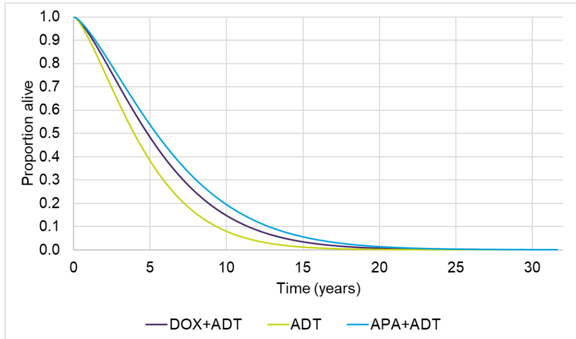
Figure 24: OS docetaxel plus ADT vs apalutamide plus ADT and ADT alone
