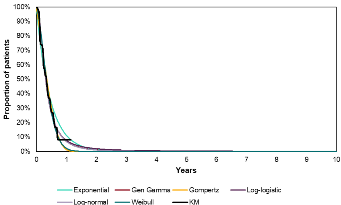
Figure 21: Parametric curve fits – LUME-Lung – PFS
