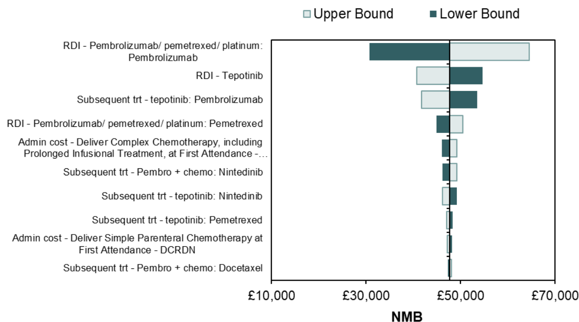
Figure 8: Tornado plot – tepotinib versus pembrolizumab + pemetrexed + platinum (WTP = £30,000)
