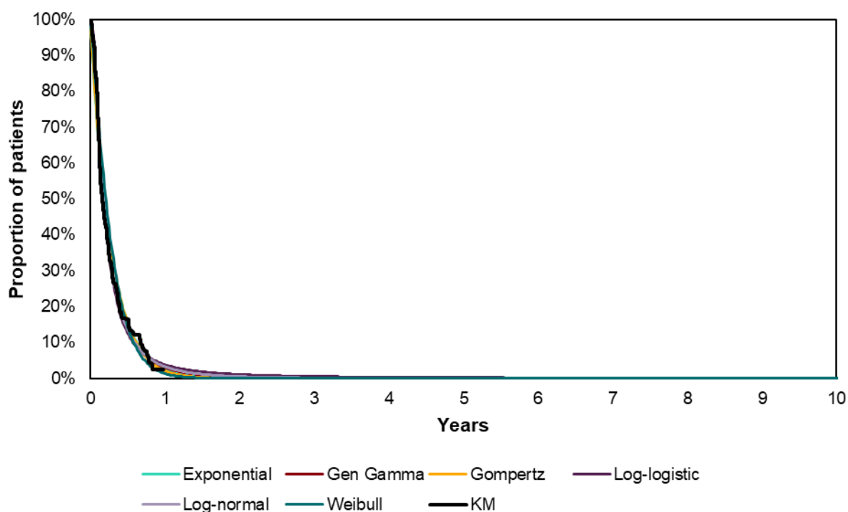
Figure 16: Parametric curve fits – Fossella et al – PFS
