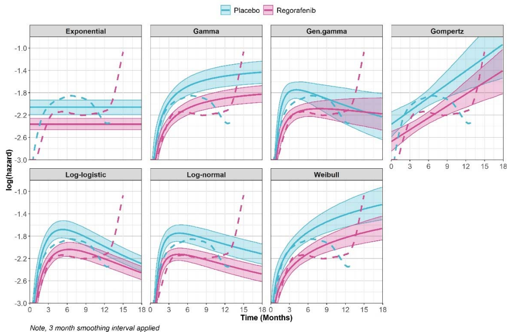
Figure B6.10: Log smoothed hazard versus time – pooled CORRECT and CONCUR OS data
