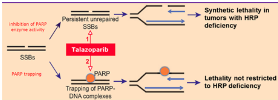
Figure 4. Talazoparib Dual Mechanism of Action.
